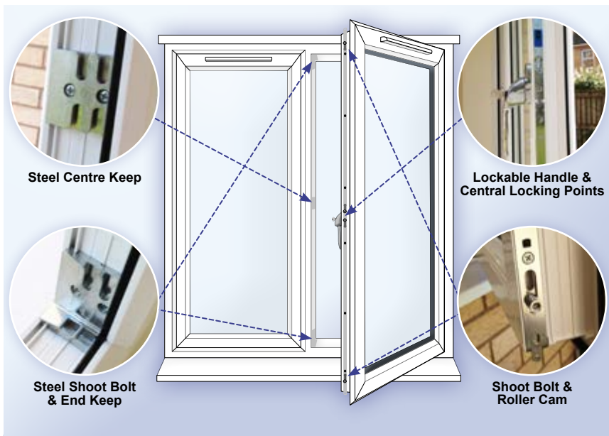
Diagram 3: Window multi-point high security lock
