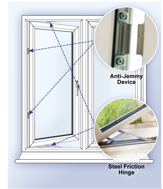
Diagram 2: Window security features
